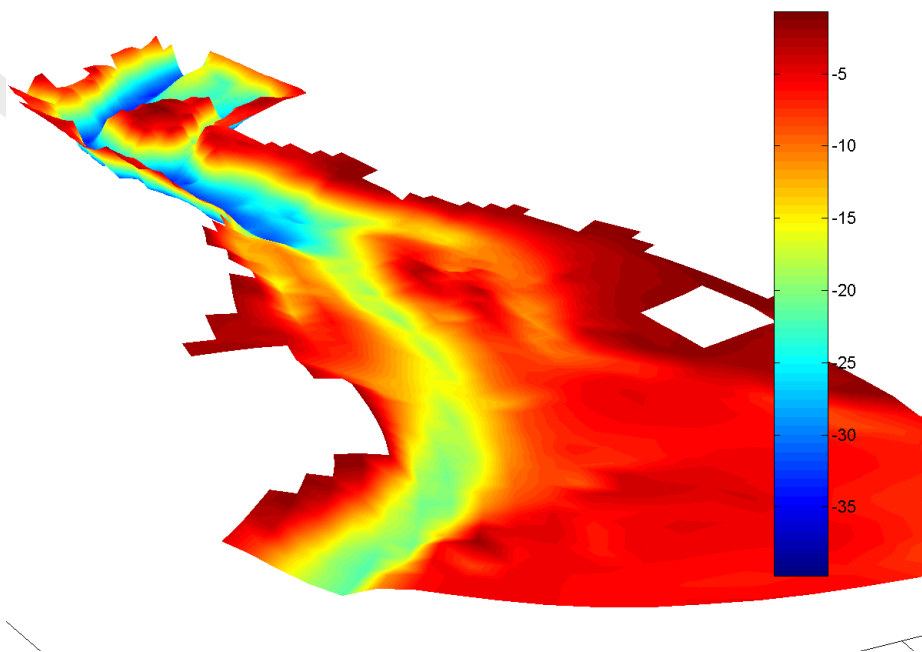
Figure 3.1: Example QUICKPLOT figure: 3D view of bed level
