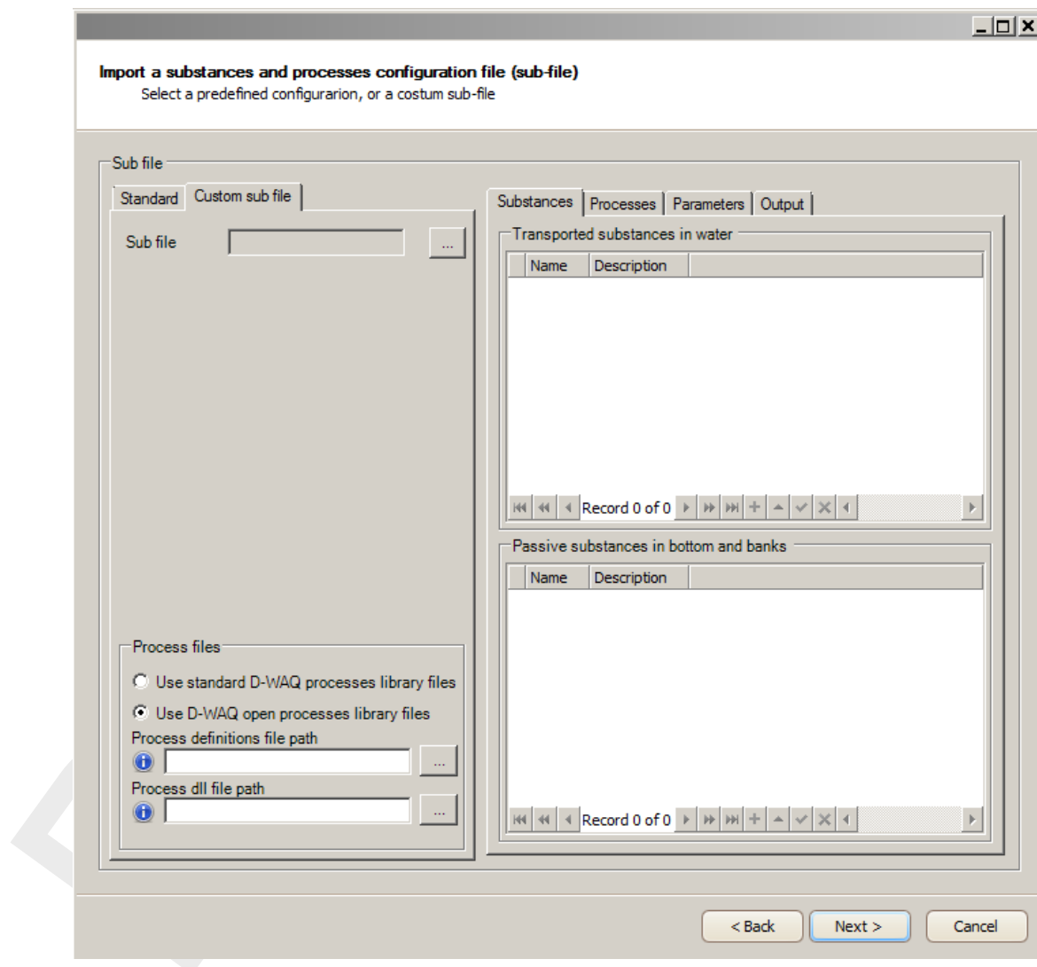
Figure 4.7: Substances file import wizard
