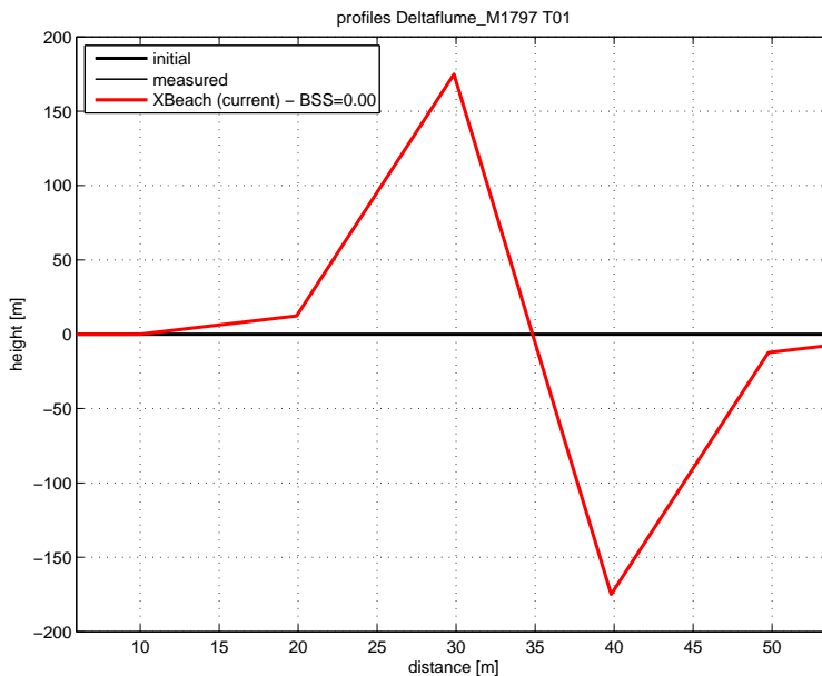
Figure 4.1: Final profile of test T01
