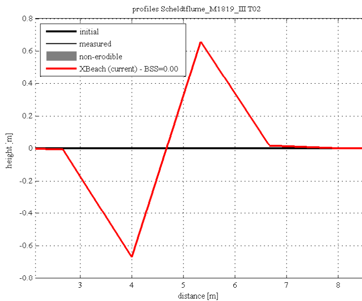
Figure 5.1: Final profile of test T02
