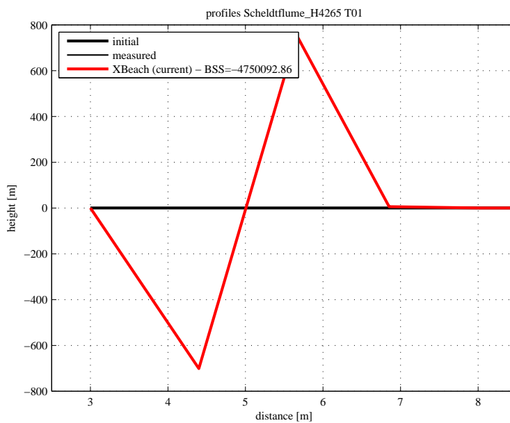
Figure 4.94: Final profile of test T01
