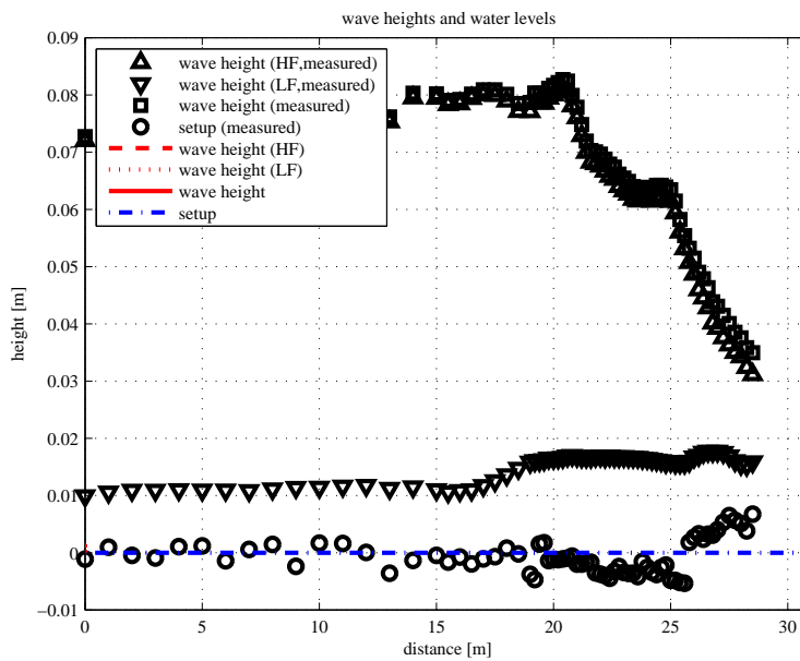
Figure 3.5: Wave height transformations during Boers 1C experiment for XBeach in surf-beat mode.
