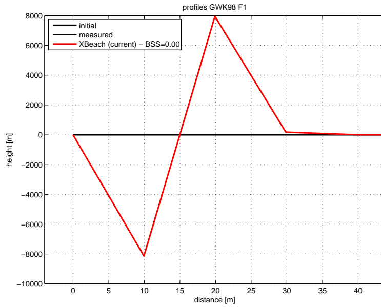
Figure 4.23: Final profile of test F1
