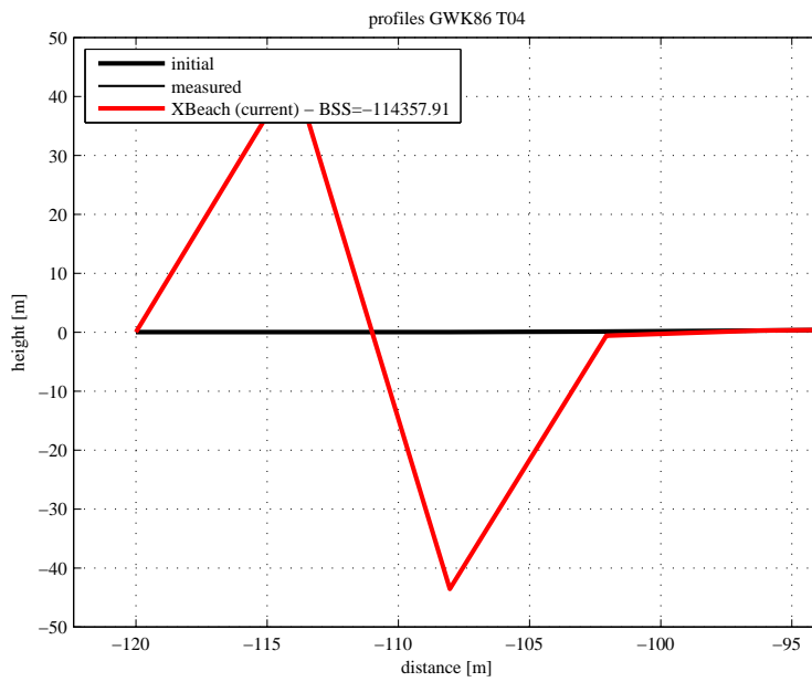
Figure 4.17: Final profile of test T04
