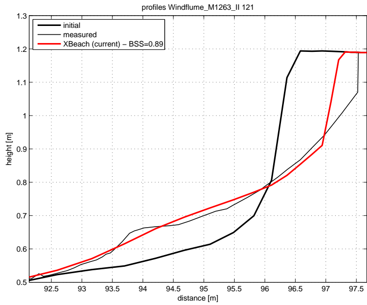
Figure 4.63: Final profile of test 121
