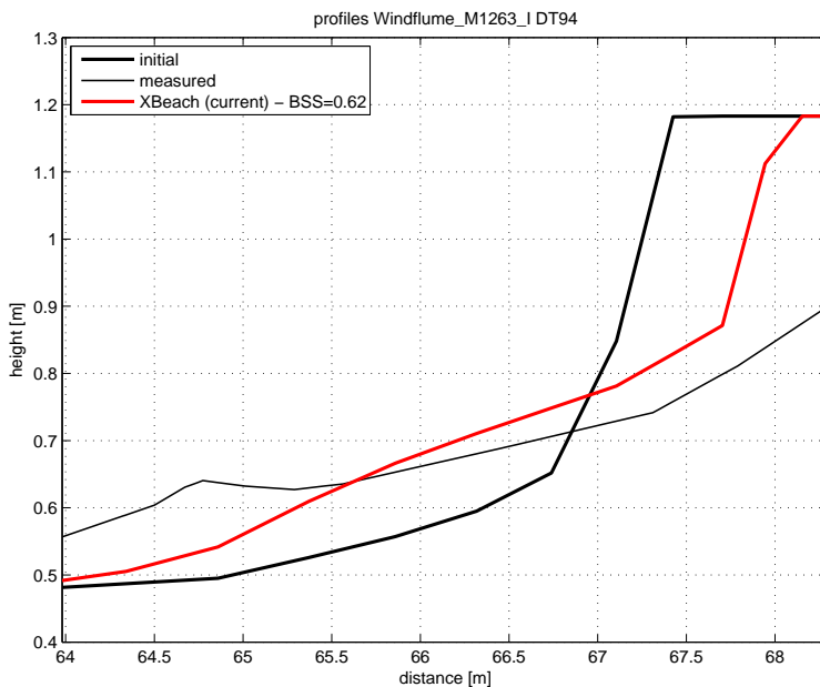
Figure 4.57: Final profile of test DT94
