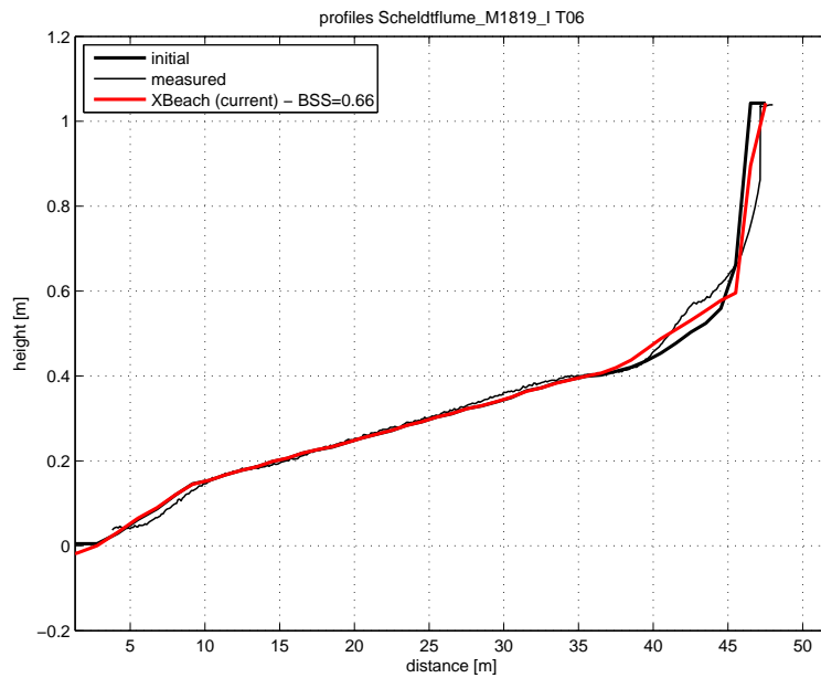
Figure 4.76: Final profile of test T06
