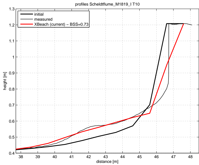
Figure 4.80: Final profile of test T10
