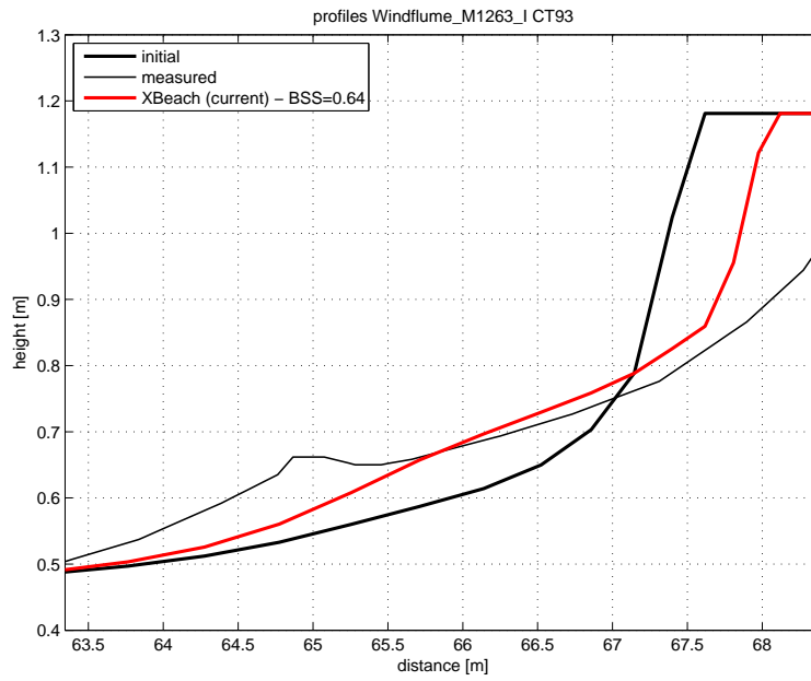
Figure 4.51: Final profile of test CT93
