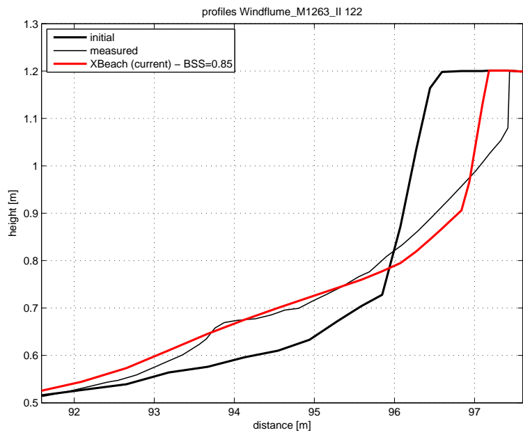
Figure 4.64: Final profile of test 122
