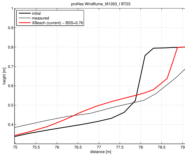
Figure 4.34: Final profile of test BT23
