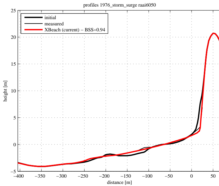
Figure 4.103: Final profile of raai 6050
