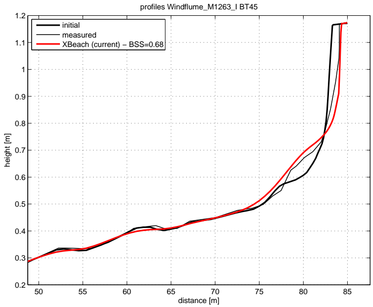
Figure 4.37: Final profile of test BT45
