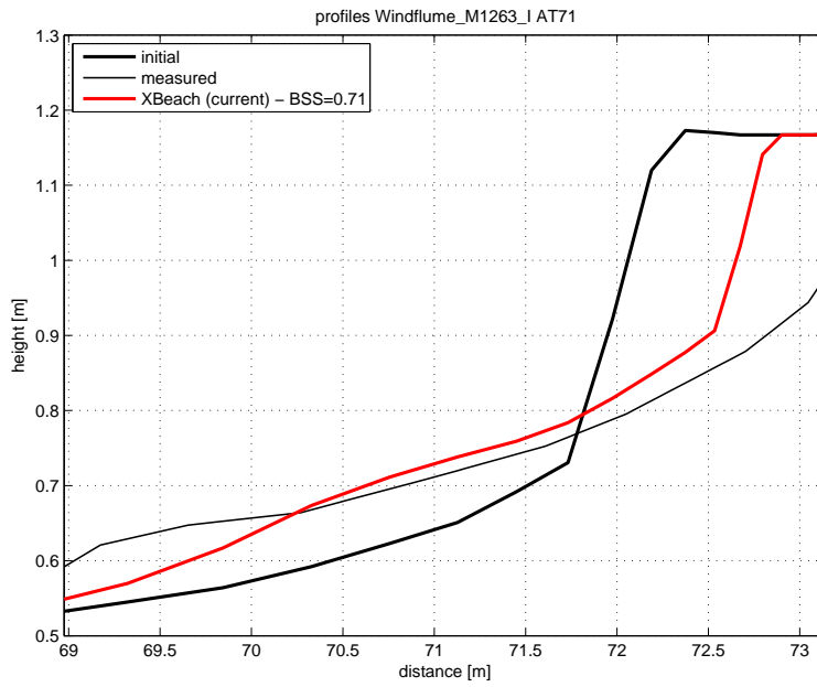
Figure 4.28: Final profile of test AT71
