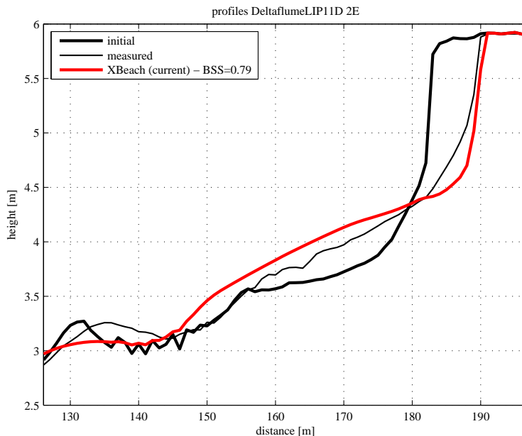
Figure 4.7: Final profile of test 2e
