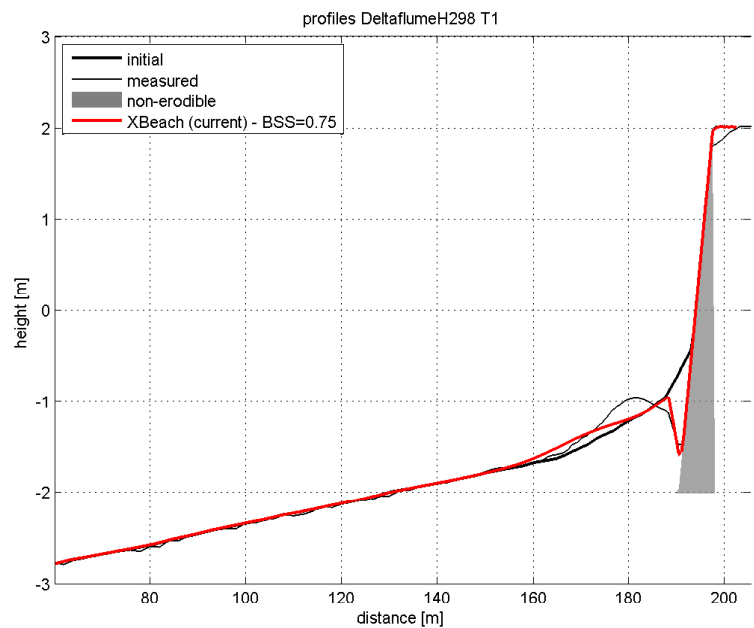
Figure 5.5: Final profile of test 1
