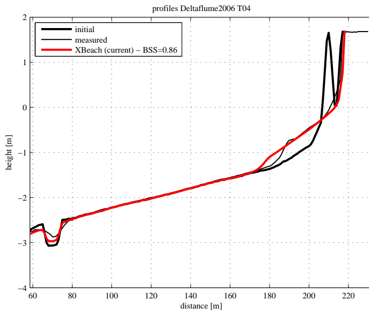
Figure 4.11: Final profile of test T04
