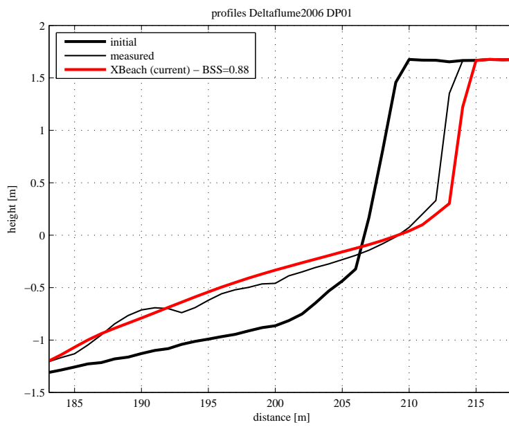
Figure 4.12: Final profile of test DP01
