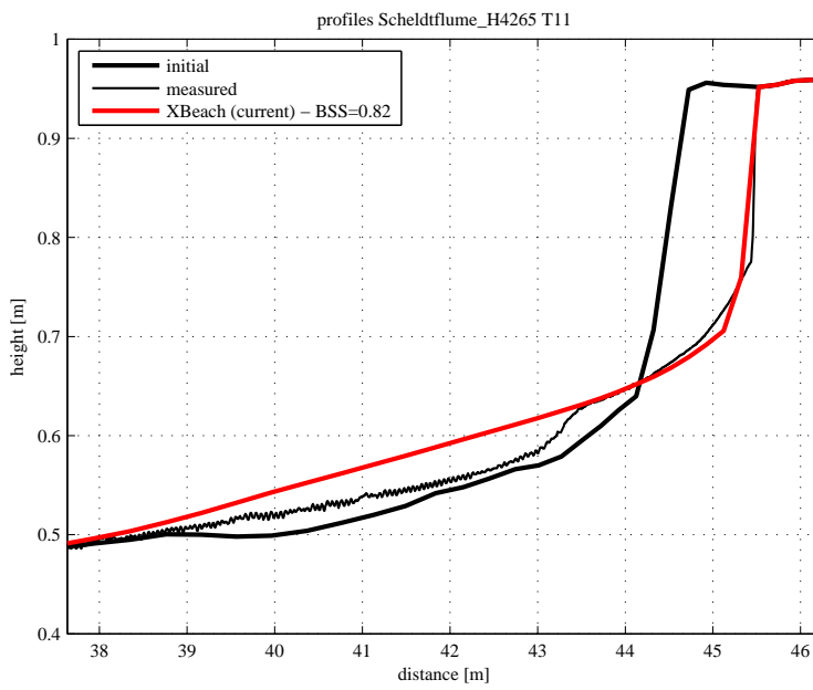
Figure 4.98: Final profile of test T011
