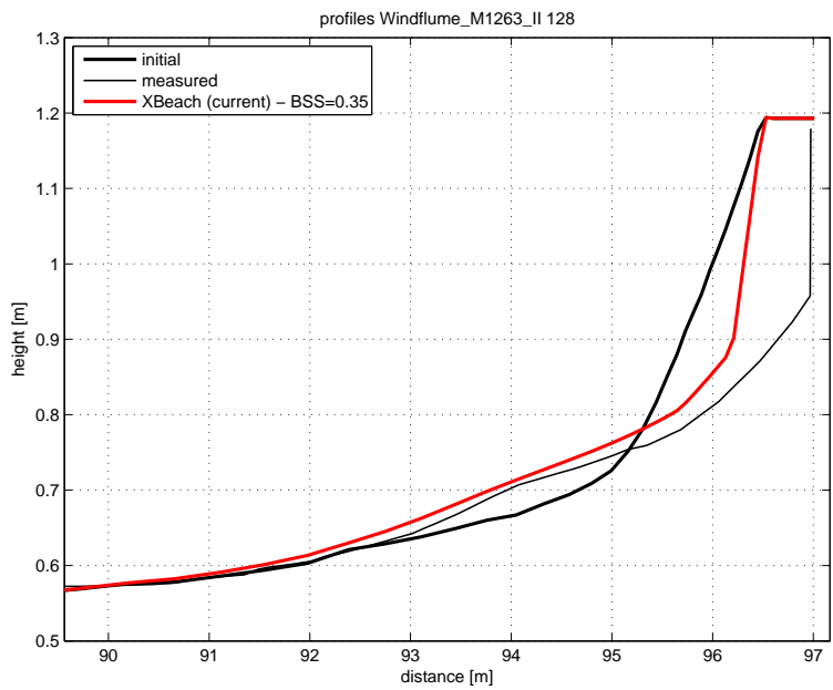
Figure 4.70: Final profile of test 128
