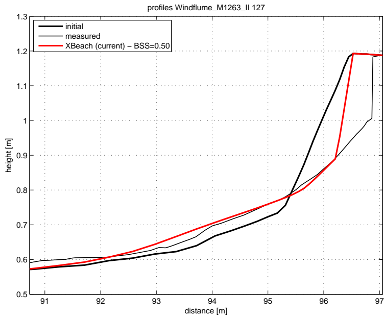
Figure 4.69: Final profile of test 127
