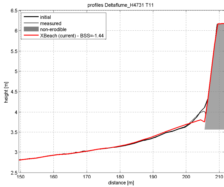
Figure 5.8: Final profile of test 11
