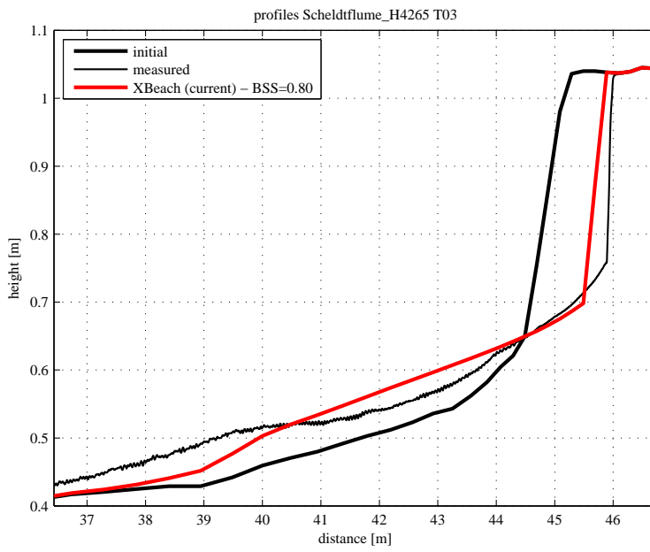
Figure 4.97: Final profile of test T03
