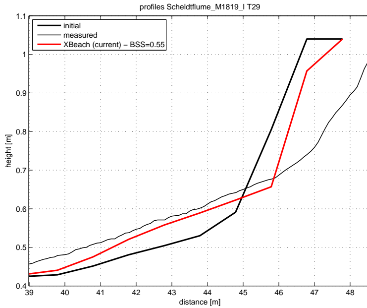
Figure 4.93: Final profile of test T29
