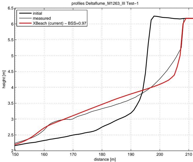
Figure 4.2: Final profile of test 1
