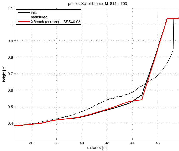
Figure 4.73: Final profile of test T03
