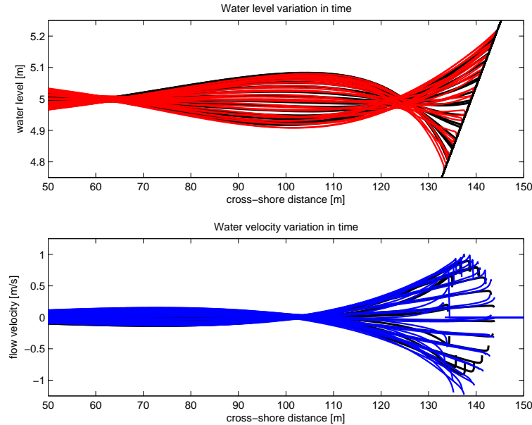
Figure 3.3: Snapshots of water level and velocity
