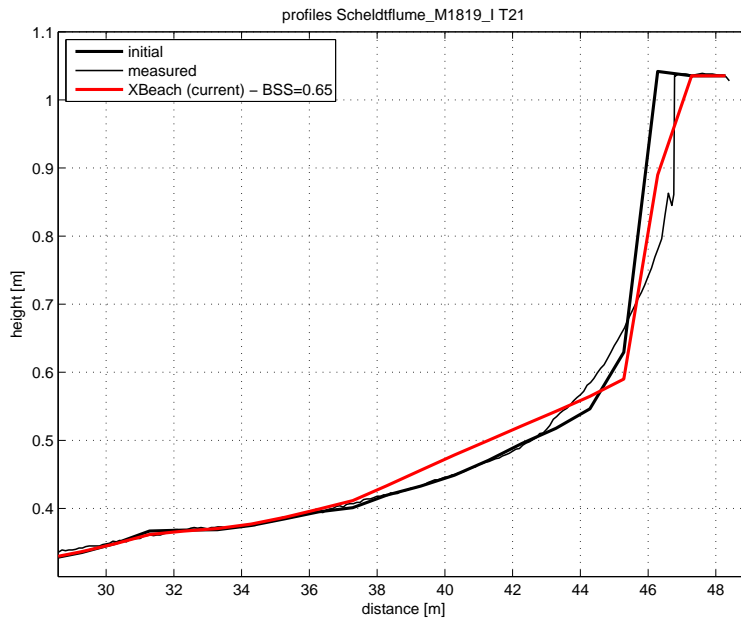
Figure 4.85: Final profile of test T21
