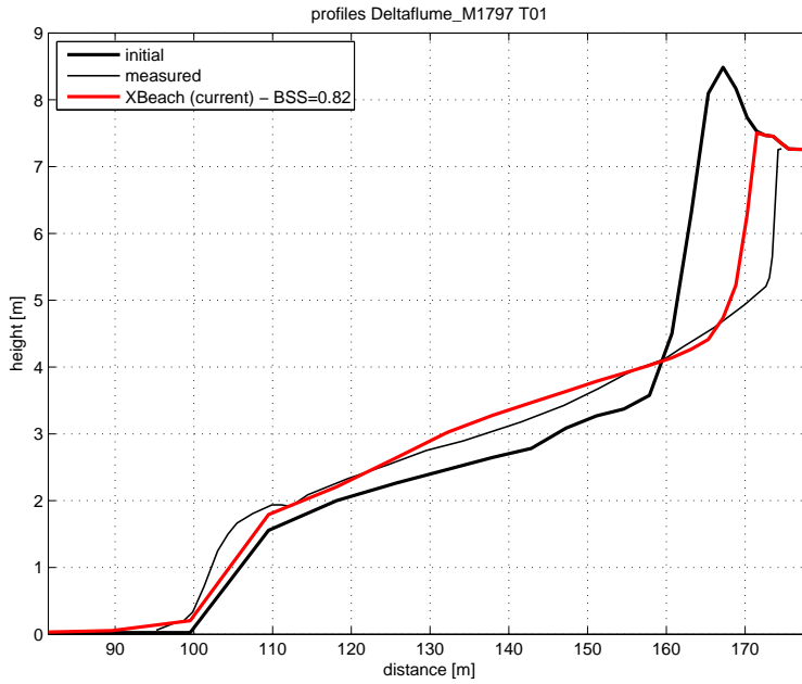
Figure 4.1: Final profile of test T01
