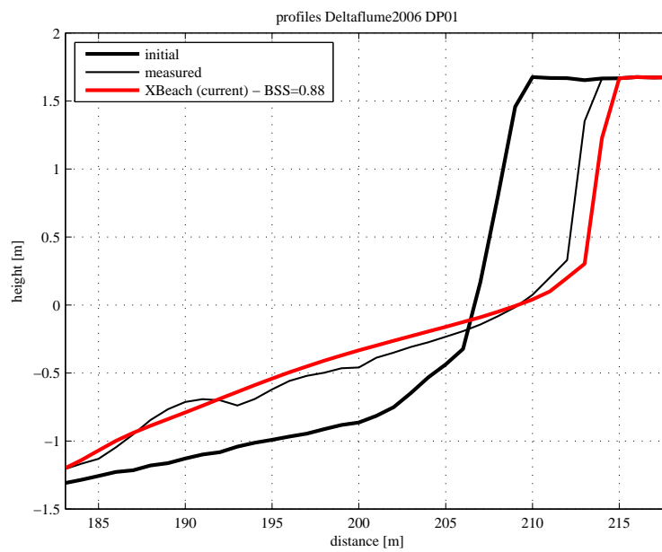
Figure 4.12: Final profile of test DP01
