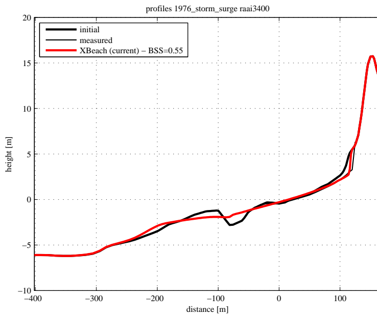
Figure 4.102: Final profile of raai 3400
