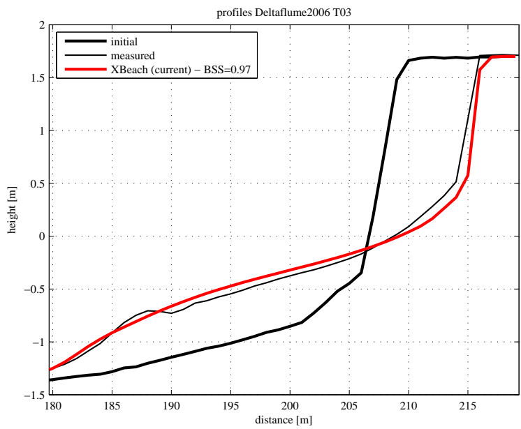
Figure 4.10: Final profile of test T03
