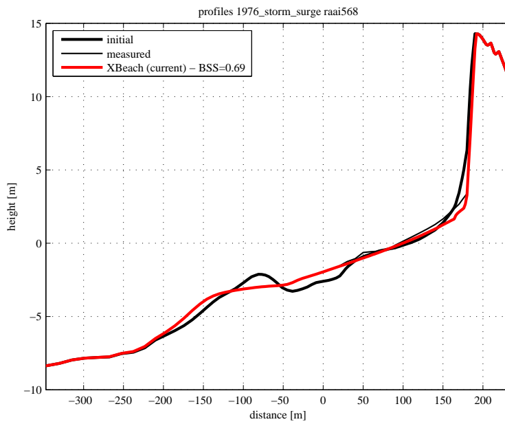
Figure 4.101: Final profile of raai 568
