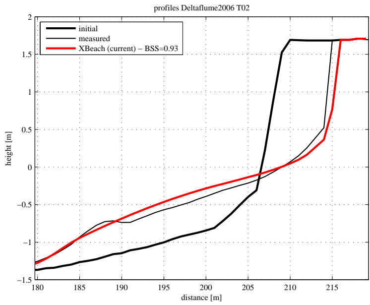
Figure 4.9: Final profile of test T02
