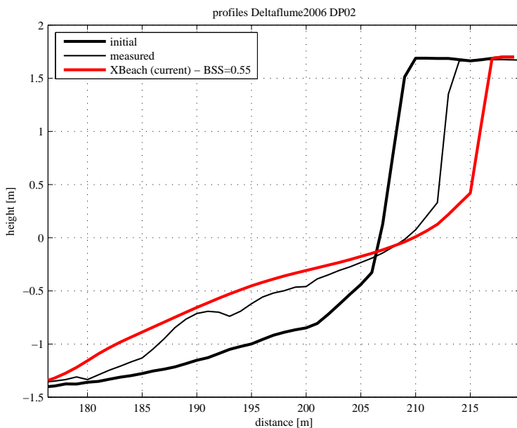
Figure 4.13: Final profile of test DP02
