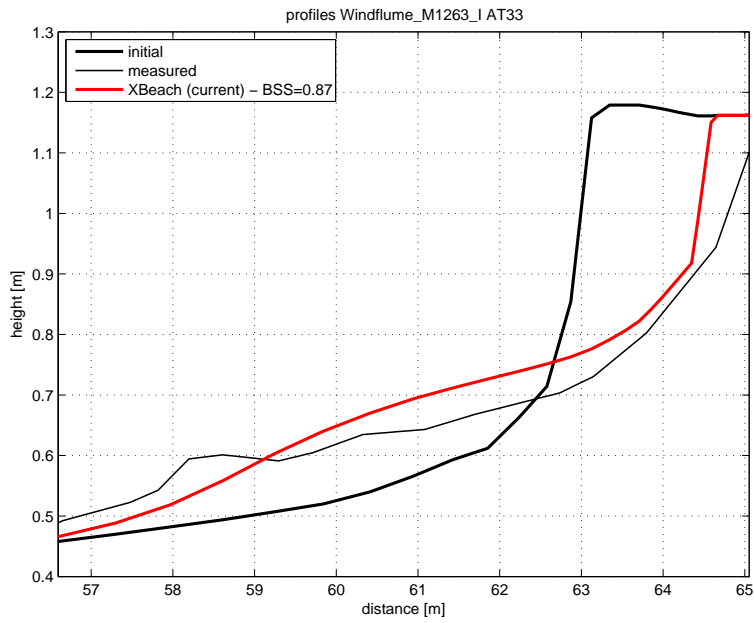
Figure 4.25: Final profile of test AT33
