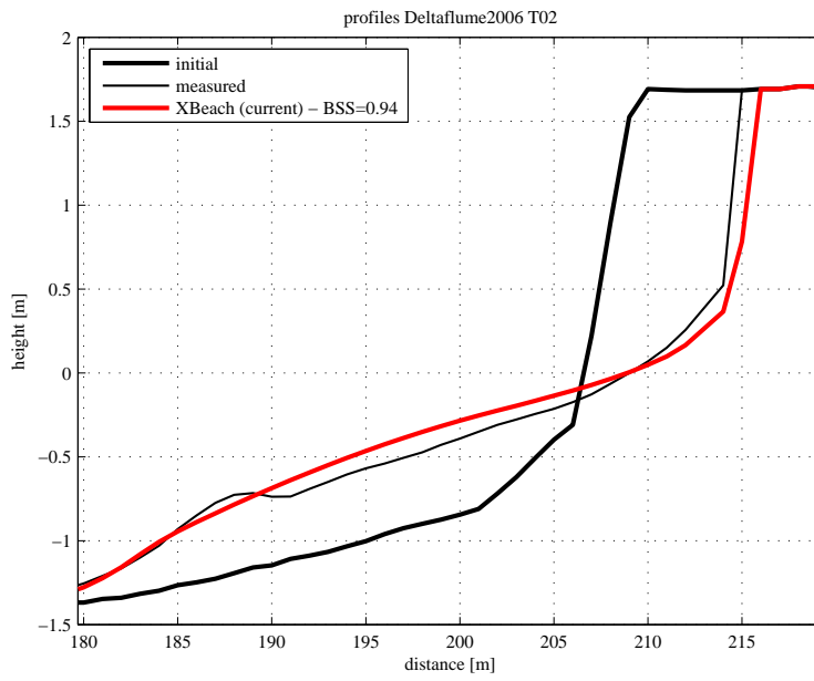
Figure 4.9: Final profile of test T02
