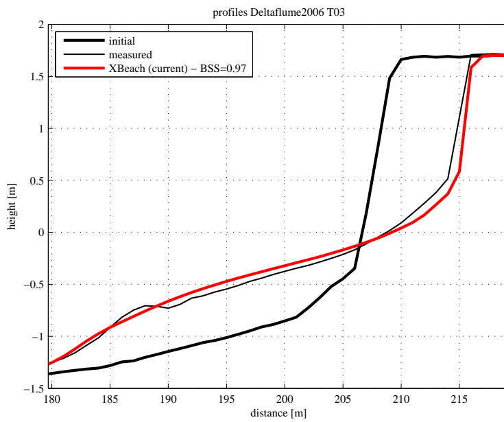
Figure 4.10: Final profile of test T03
