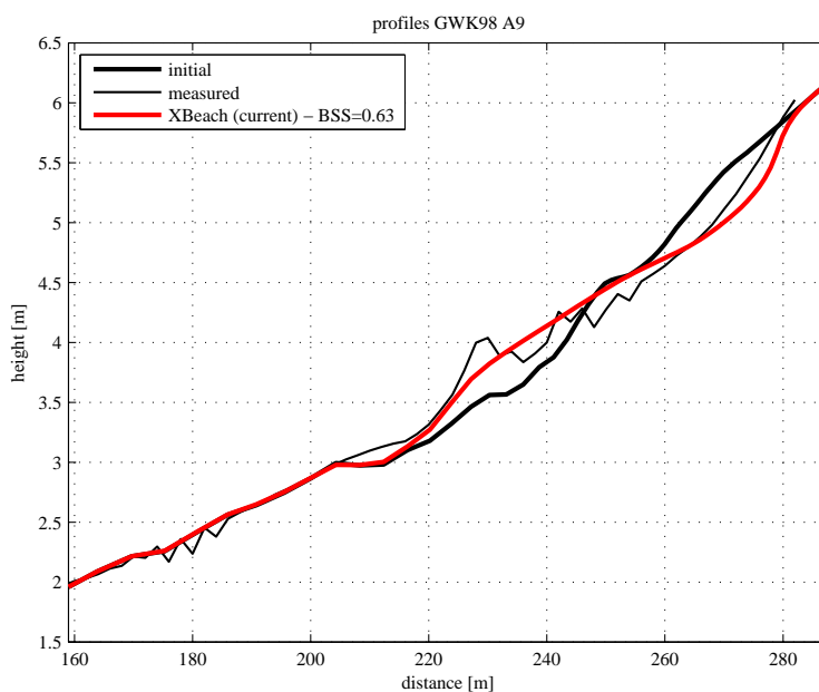
Figure 4.20: Final profile of test A9
