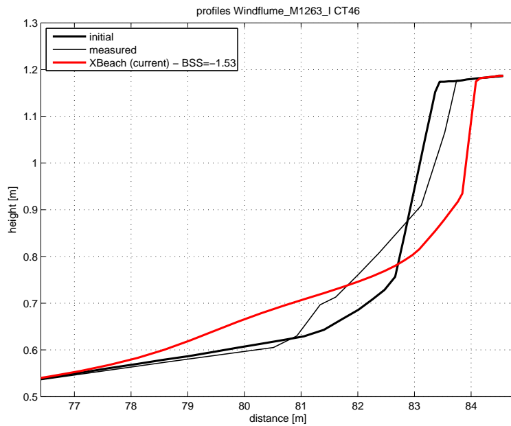
Figure 4.48: Final profile of test CT46
