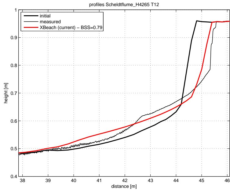
Figure 4.99: Final profile of test T012
