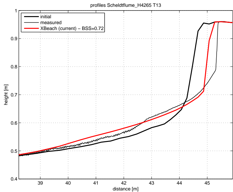
Figure 4.100: Final profile of test T013
