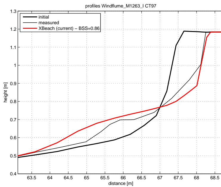
Figure 4.52: Final profile of test CT97
