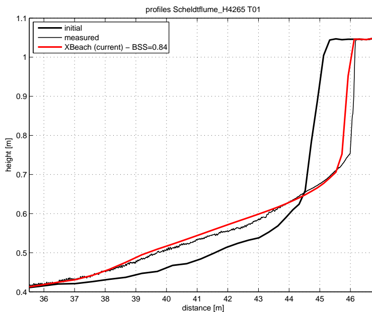
Figure 4.94: Final profile of test T01
