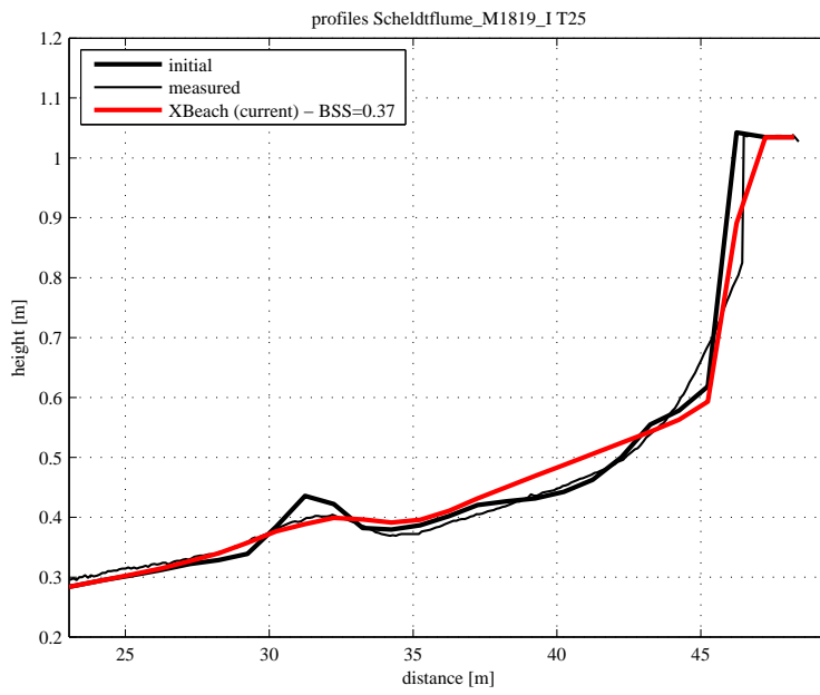
Figure 4.89: Final profile of test T25
