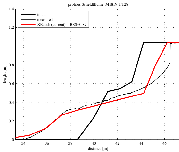
Figure 4.92: Final profile of test T28
