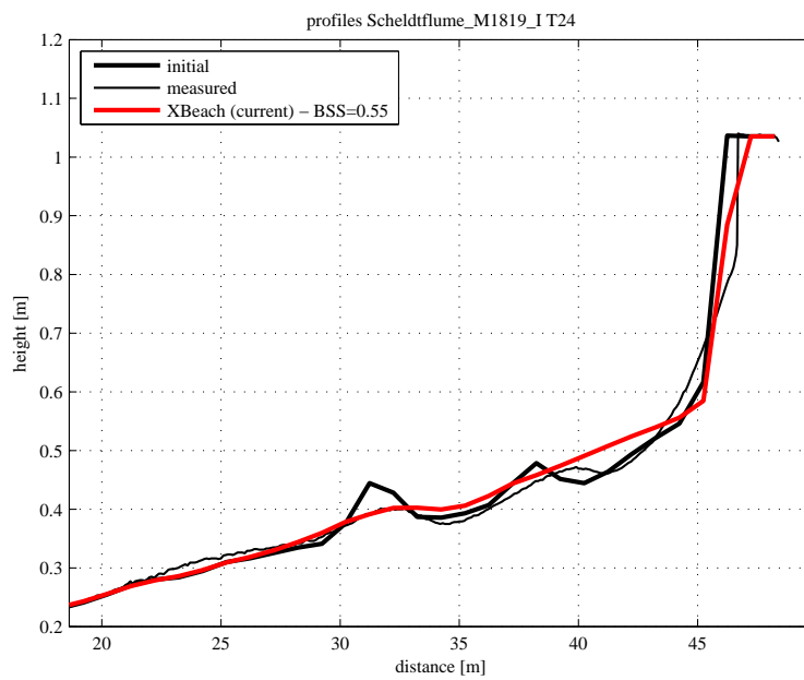
Figure 4.88: Final profile of test T24
