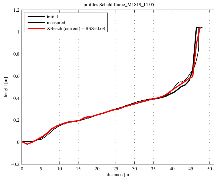
Figure 4.75: Final profile of test T05
