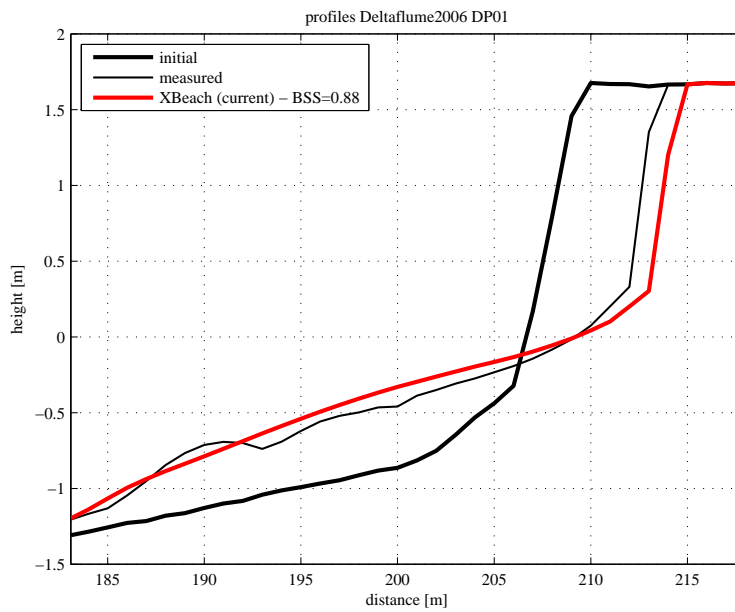
Figure 4.12: Final profile of test DP01
