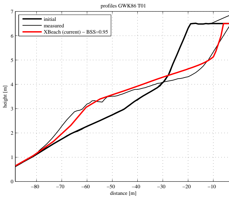
Figure 4.14: Final profile of test T01
