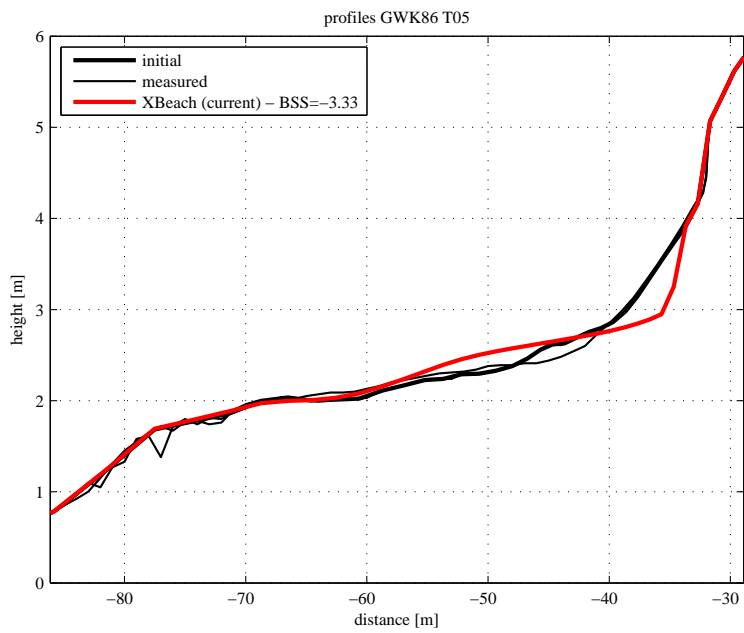
Figure 4.18: Final profile of test T05
