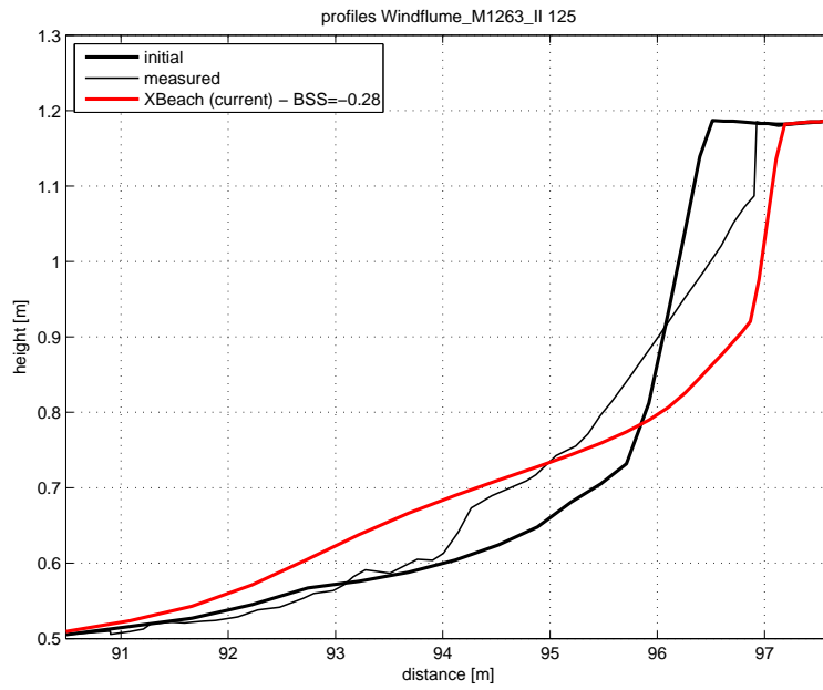
Figure 4.67: Final profile of test 125
