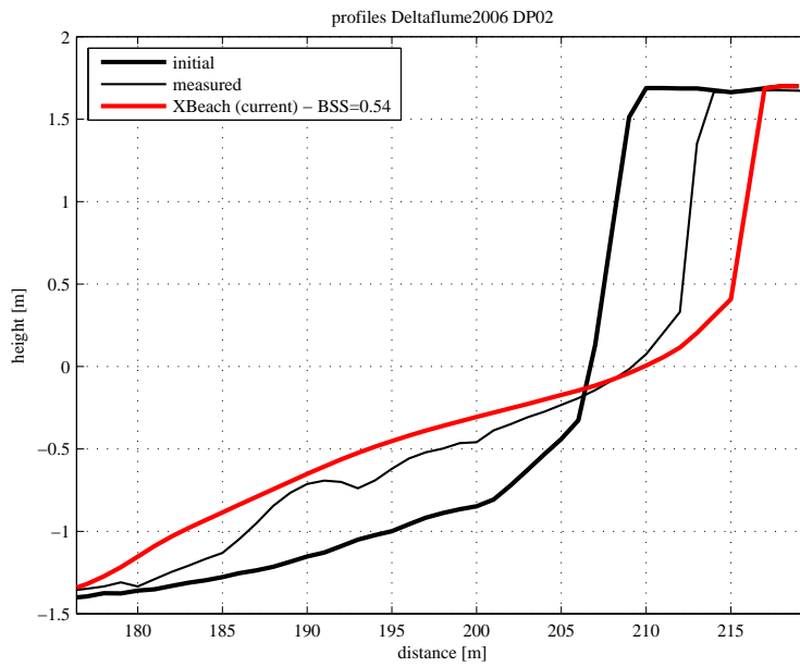
Figure 4.13: Final profile of test DP02
