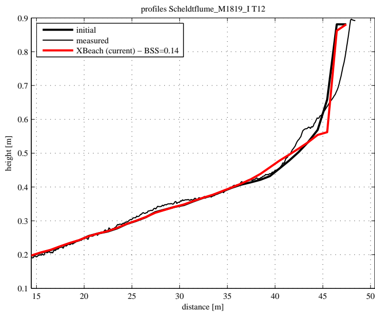
Figure 4.82: Final profile of test T12
