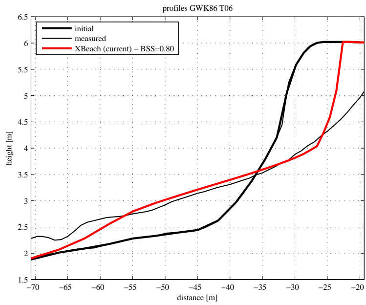
Figure 4.19: Final profile of test T06
