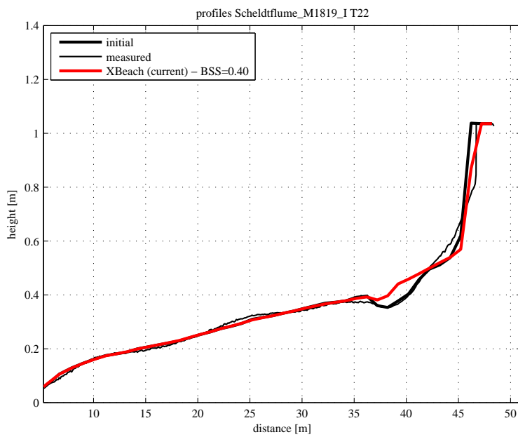
Figure 4.86: Final profile of test T22
