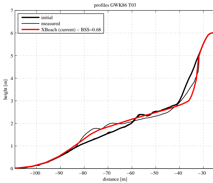
Figure 4.16: Final profile of test T03
