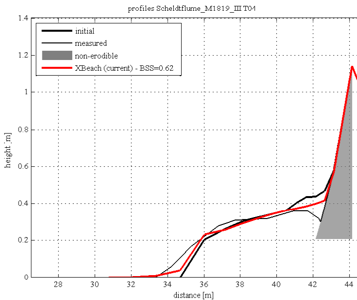
Figure 5.3: Final profile of test T04
