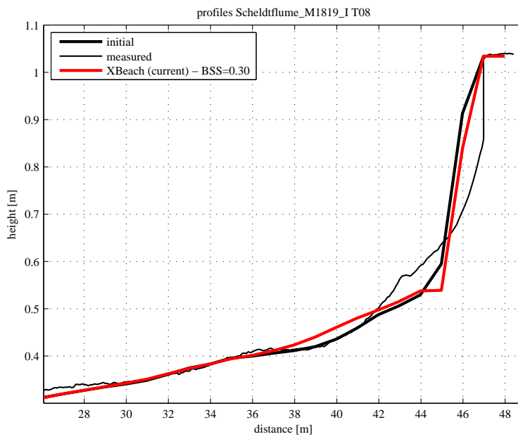
Figure 4.78: Final profile of test T08
