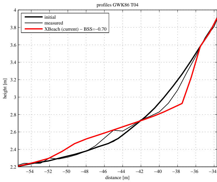
Figure 4.17: Final profile of test T04
