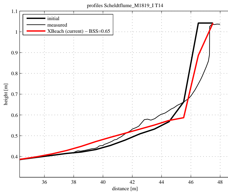
Figure 4.84: Final profile of test T14
