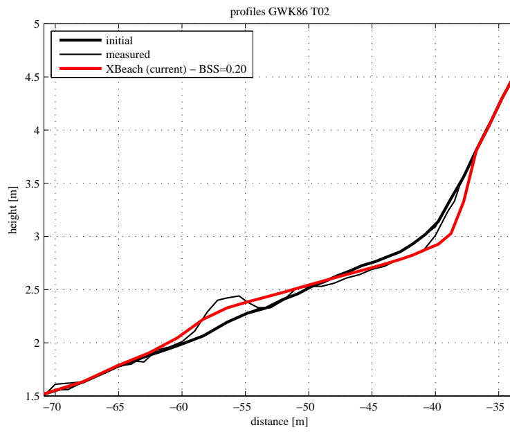
Figure 4.15: Final profile of test T02
