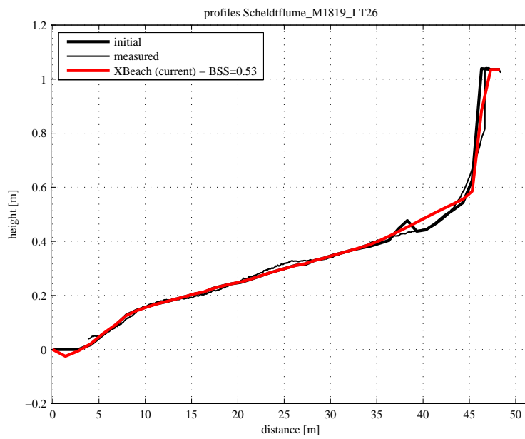
Figure 4.90: Final profile of test T26
