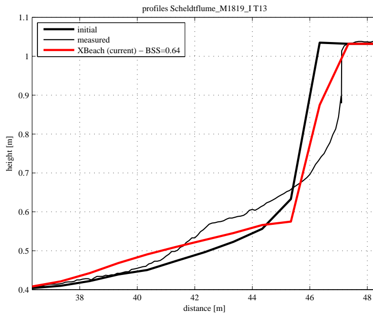
Figure 4.83: Final profile of test T13
