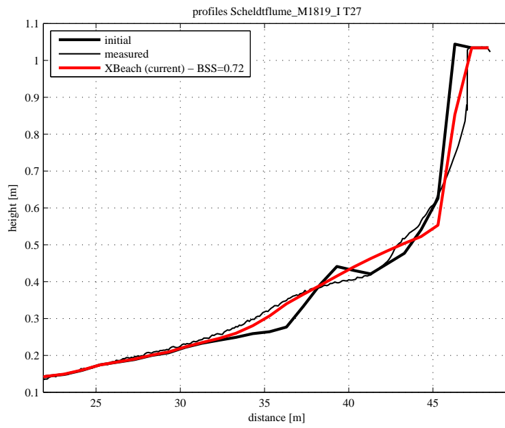
Figure 4.91: Final profile of test T27
