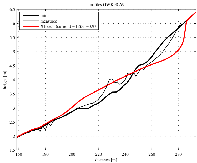
Figure 4.20: Final profile of test A9
