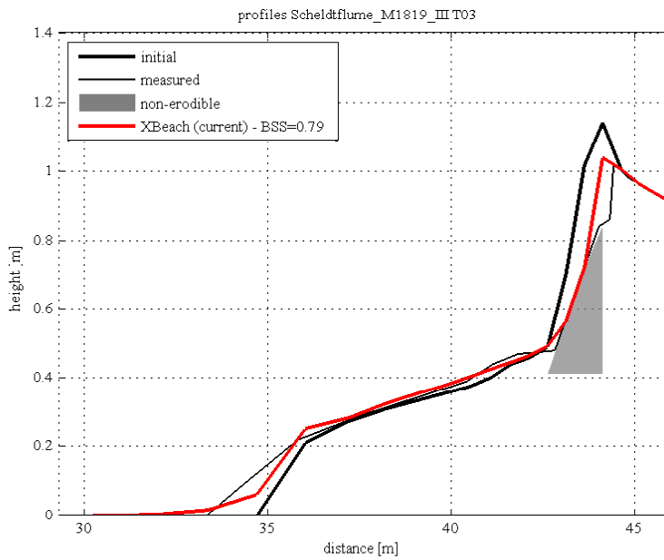
Figure 5.2: Final profile of test T03
