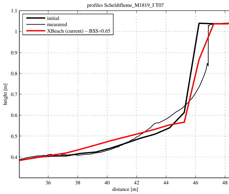
Figure 4.77: Final profile of test T07
