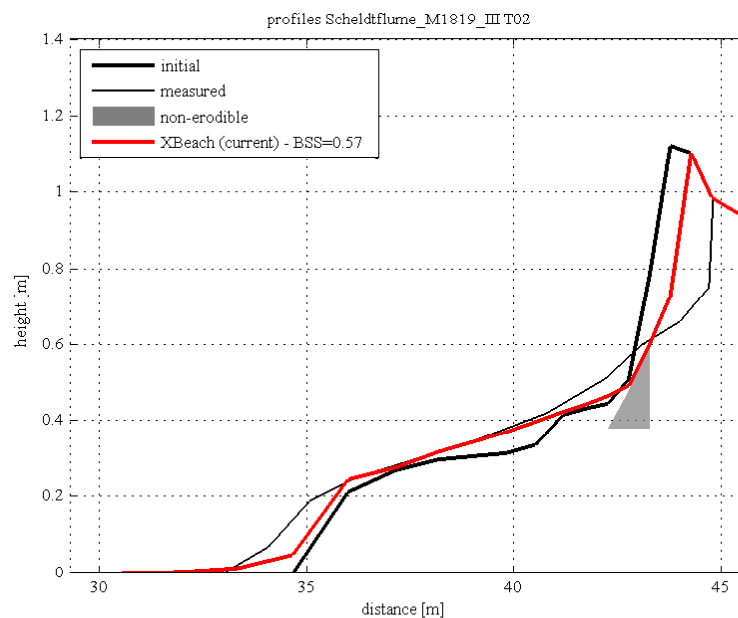
Figure 5.1: Final profile of test T02
