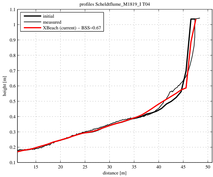
Figure 4.74: Final profile of test T04
