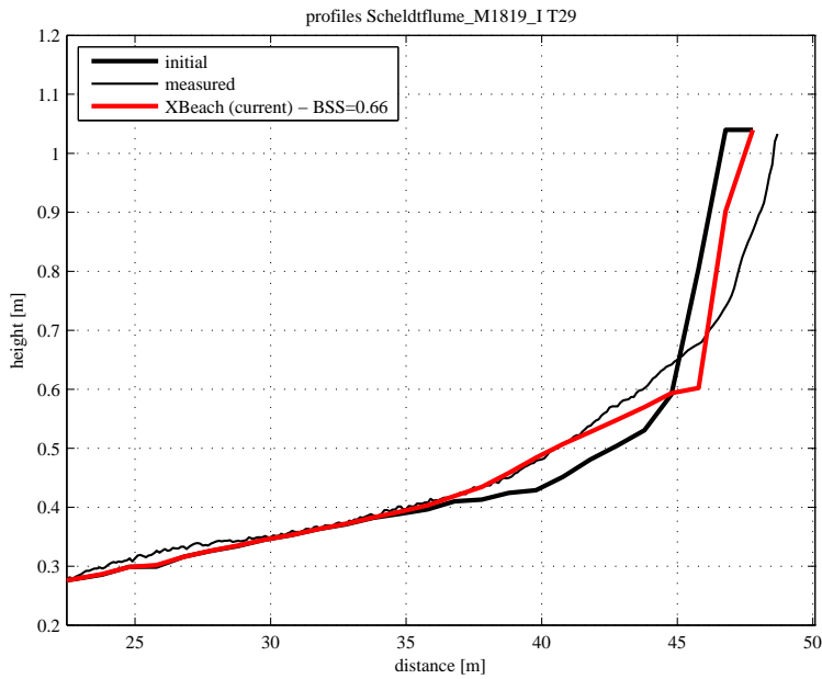
Figure 4.93: Final profile of test T29
