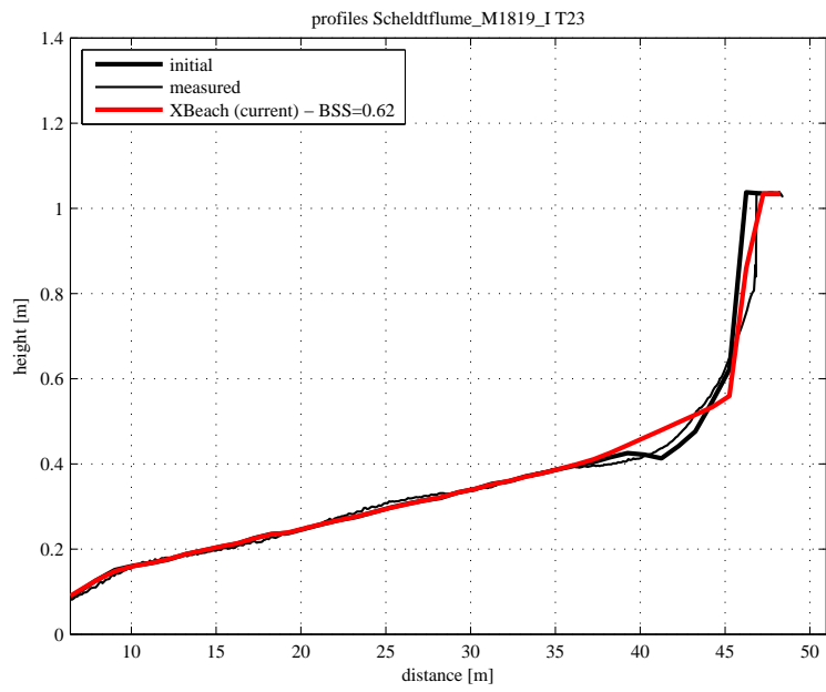
Figure 4.87: Final profile of test T23
