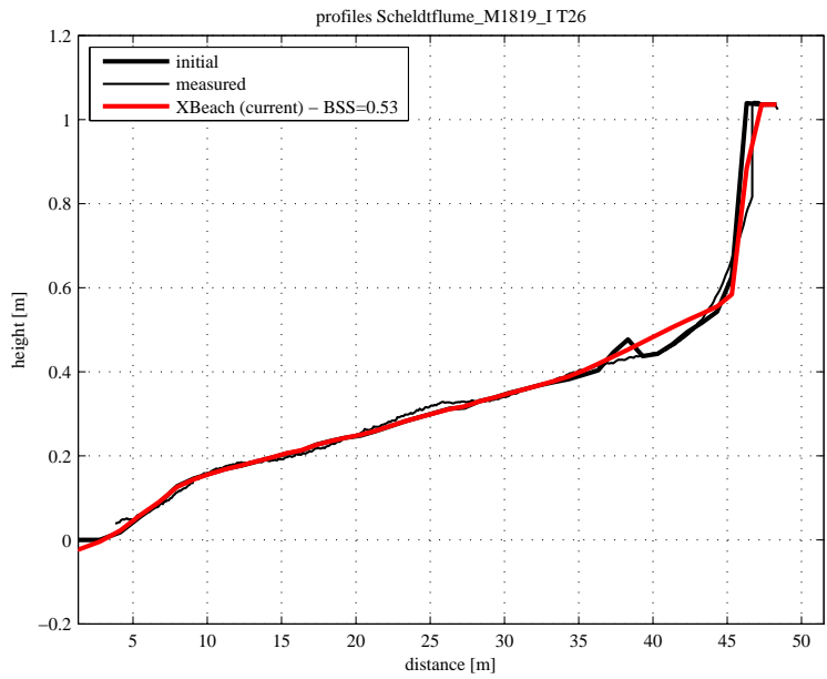
Figure 4.90: Final profile of test T26
