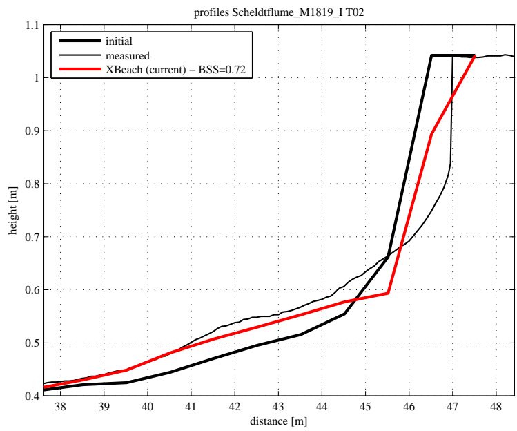
Figure 4.72: Final profile of test T02
