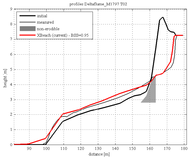
Figure 5.4: Final profile of test T02
