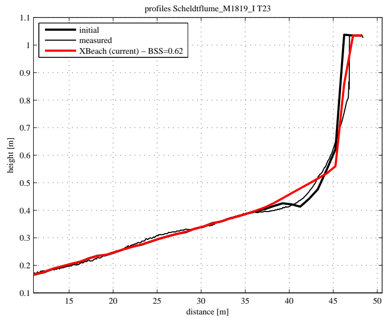
Figure 4.87: Final profile of test T23
