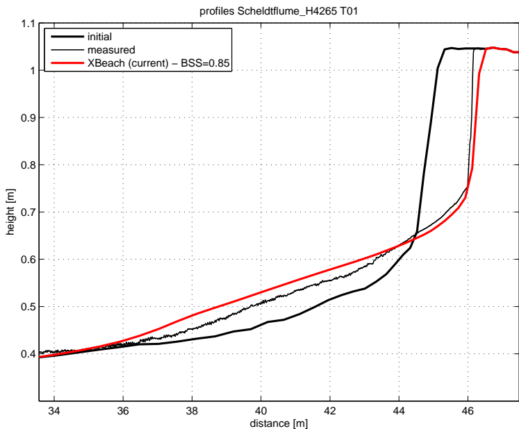
Figure 4.94: Final profile of test T01
