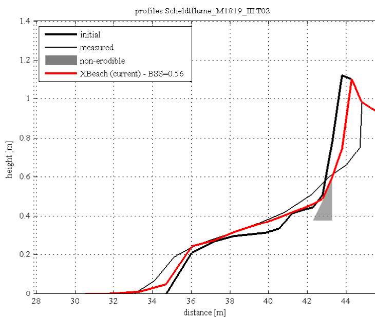
Figure 5.1: Final profile of test T02
