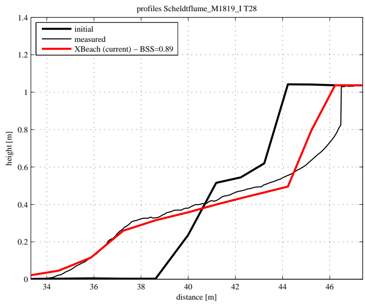
Figure 4.92: Final profile of test T28
