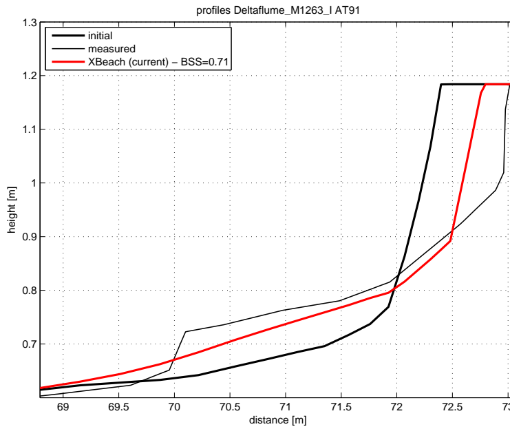
Figure 4.29: Final profile of test AT91
