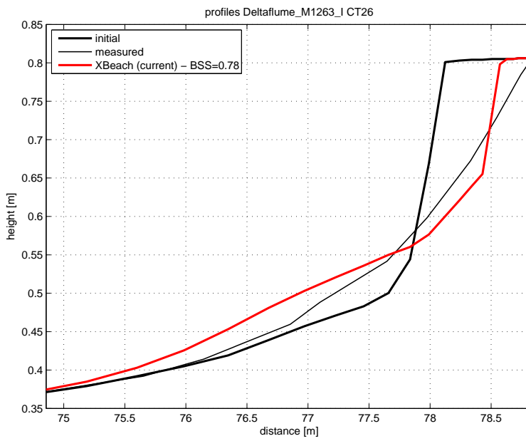
Figure 4.46: Final profile of test CT26
