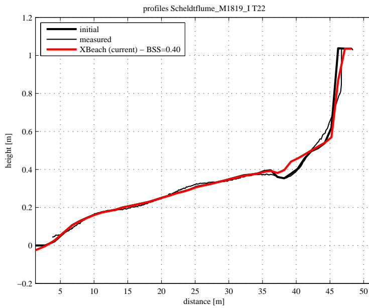
Figure 4.86: Final profile of test T22
