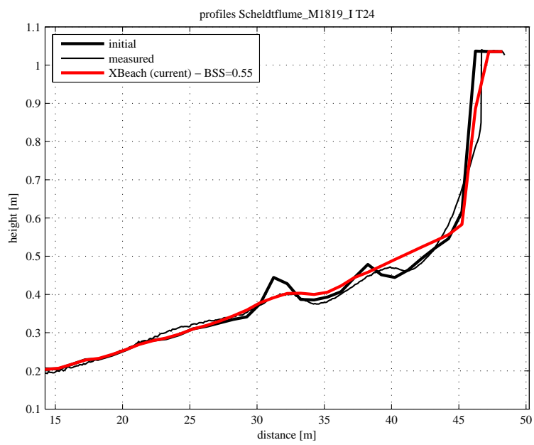
Figure 4.88: Final profile of test T24
