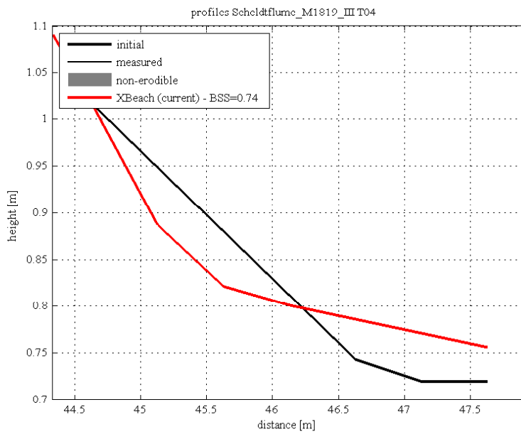
Figure 5.3: Final profile of test T04
