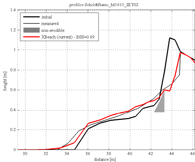
Figure 5.1: Final profile of test T02
