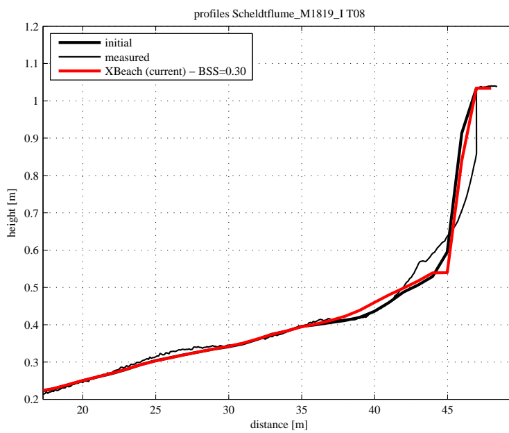
Figure 4.78: Final profile of test T08
