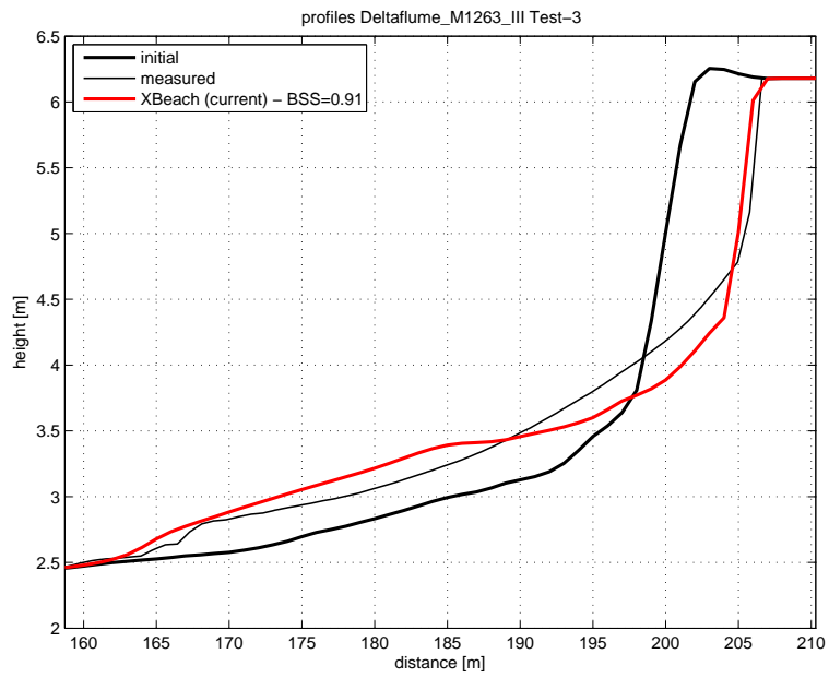
Figure 4.4: Final profile of test 3
