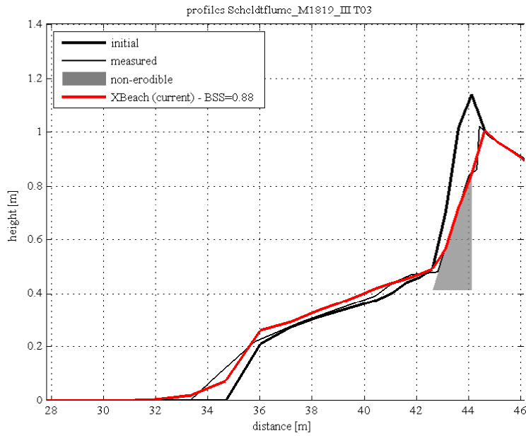
Figure 5.2: Final profile of test T03
