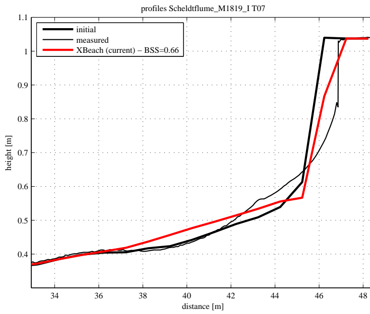
Figure 4.77: Final profile of test T07
