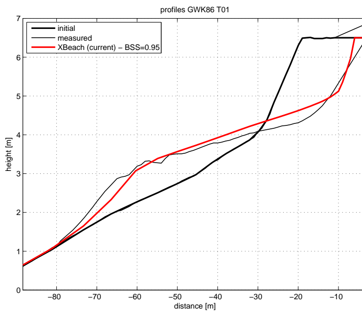
Figure 4.14: Final profile of test T01
