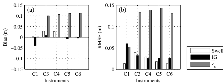
Figure 2.14: Bias and RMS error from the 1D swell duration ( 5 day) model results compared with the measured data at each site, based on the short wave heights, IG wave heights, and mean water levels.
