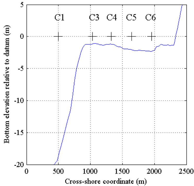
Figure 2.15: Cross-shore profile of the bathymetry along the main measurement transect with instrument locations shown.
