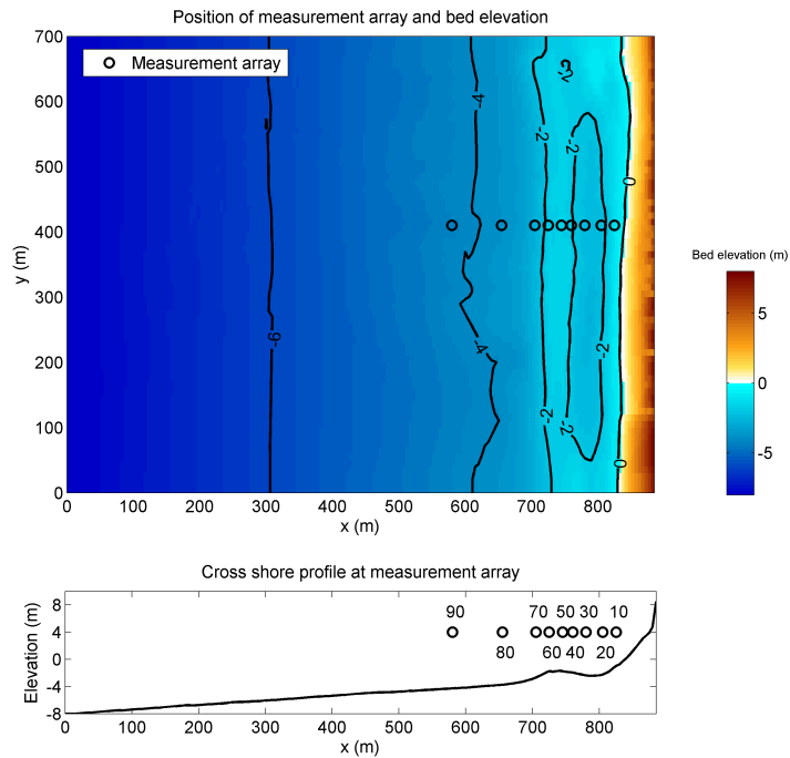
Figure 2.12: Bathymetry and measurement locations
