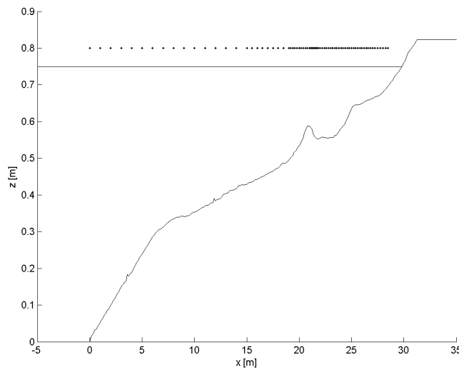
Figure 2.6: Locations of surface elevation measurements
