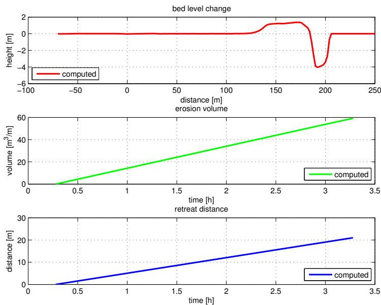
Figure 3.19: Development of erosion volumes during test 5
