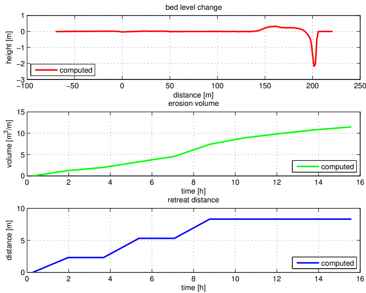
Figure 3.18: Development of erosion volumes during test 4
