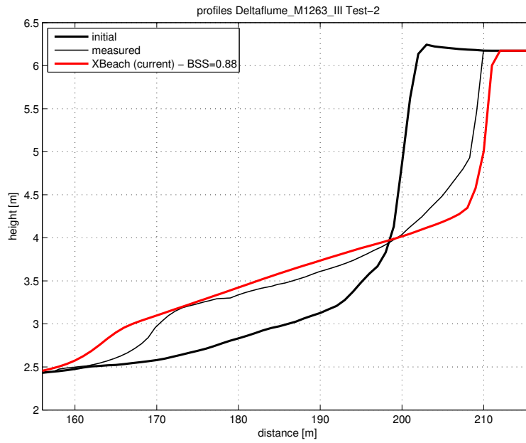
Figure 3.10: Profile development during test 2
