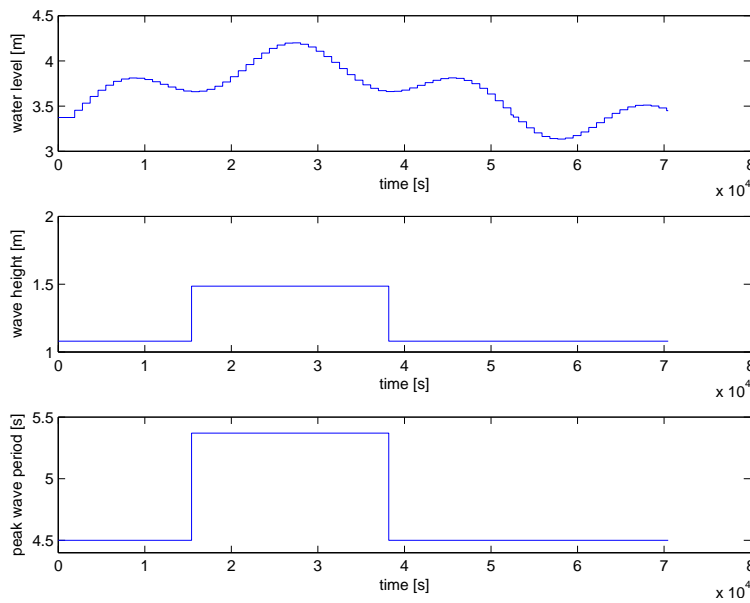
Figure 4.5: Boundary conditions for test 3
