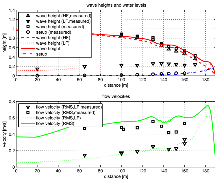
Figure 4.21: Hydrodynamics during test 2E
