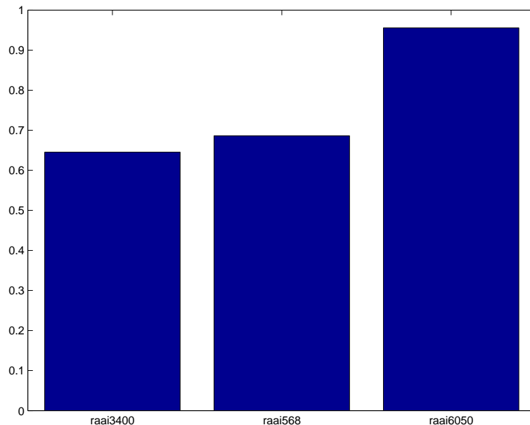
Figure 5.5: Overview of Brier Skill Scores
