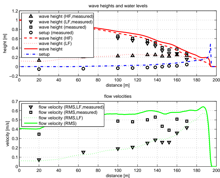
Figure 4.24: Hydrodynamics during test 1B
