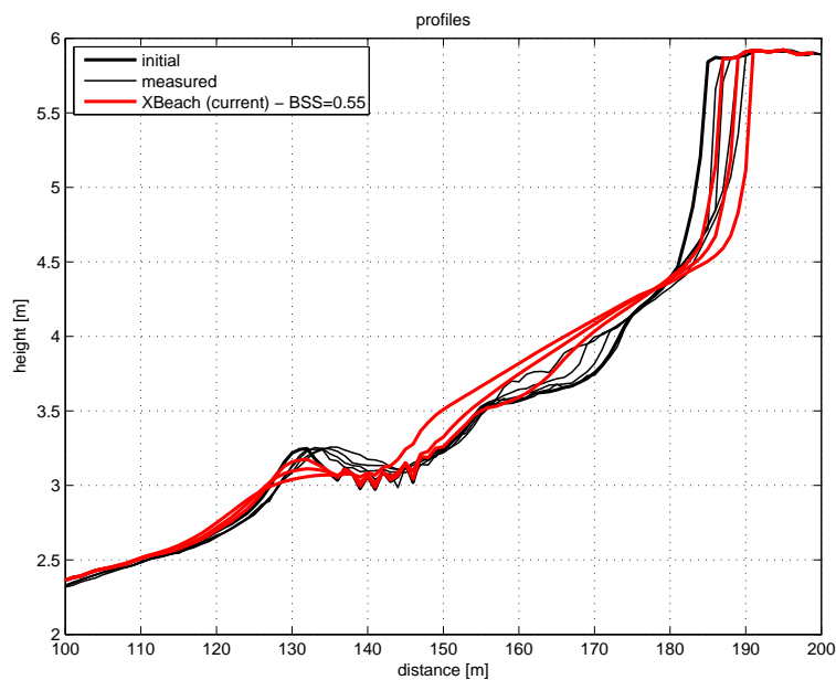
Figure 4.23: Profile development during test 2E
