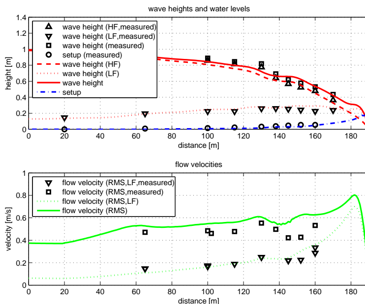
Figure 4.21: Hydrodynamics during test 2E
