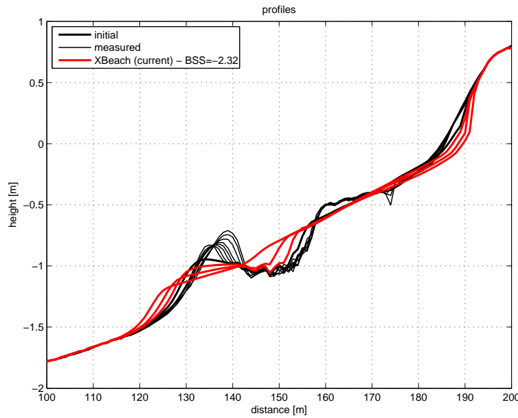
Figure 4.27: Profile development during test 1C
