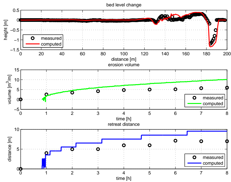
Figure 4.22: Morphodynamics during test 2E
