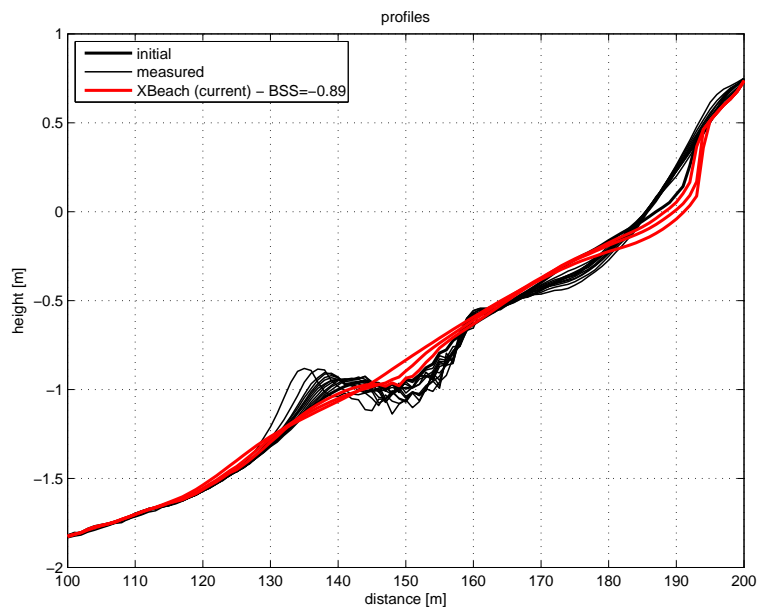
Figure 4.26: Profile development during test 1B
