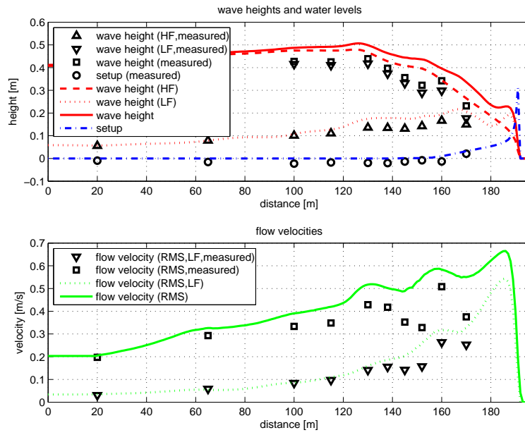
Figure 4.25: Hydrodynamics during test 1C
