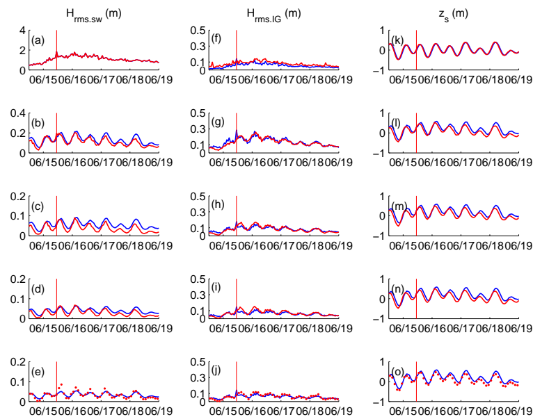
Figure 3.12: Comparison between the 1D model results (blue) and measured data (red) for the duration of the 5 day swell event. (a,f,k) are for instrument C1, (b,g,l) C3, (c,h,m) C4, (d,i,n) C5 and (e,j,o) C6. The peak of the storm is indicated by the red vertical line. Note the large reduction in vertical scale between C1 and the reef sites C3-C6.
