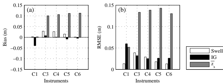
Figure 3.13: Bias and RMS error from the 1D swell duration ( 5 day) model results compared with the measured data at each site, based on the short wave heights, IG wave heights, and mean water levels.
