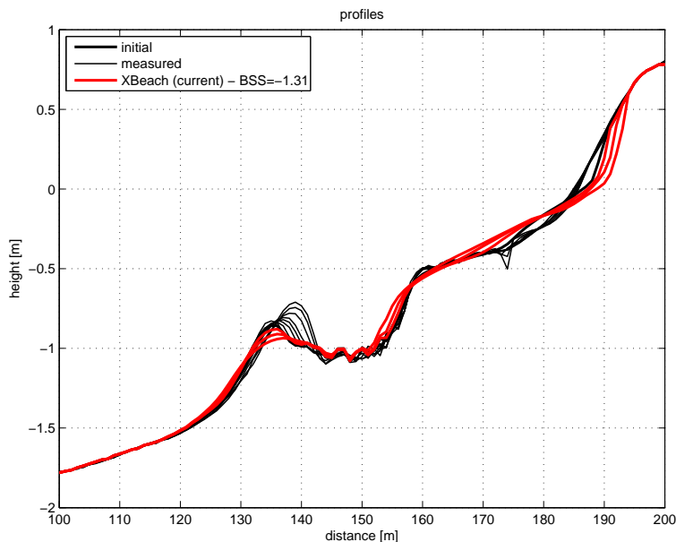
Figure 4.27: Profile development during test 1C
