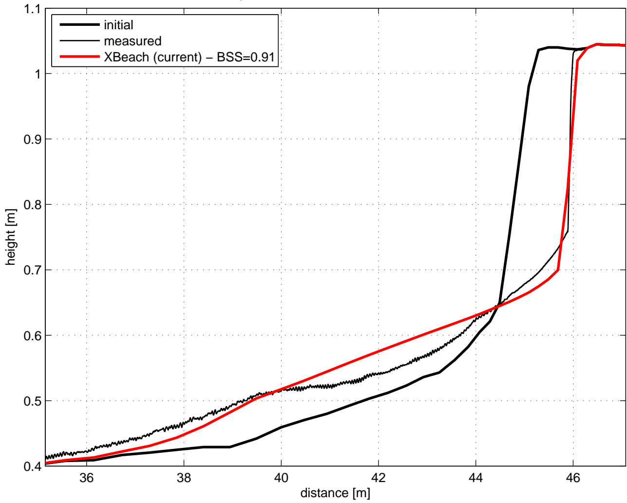
profiles Scheldtflume_H4265 T03
