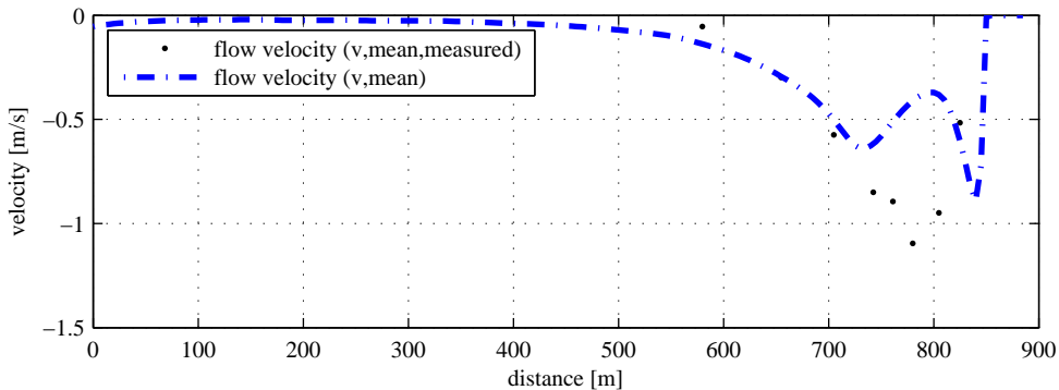
flow velocities
