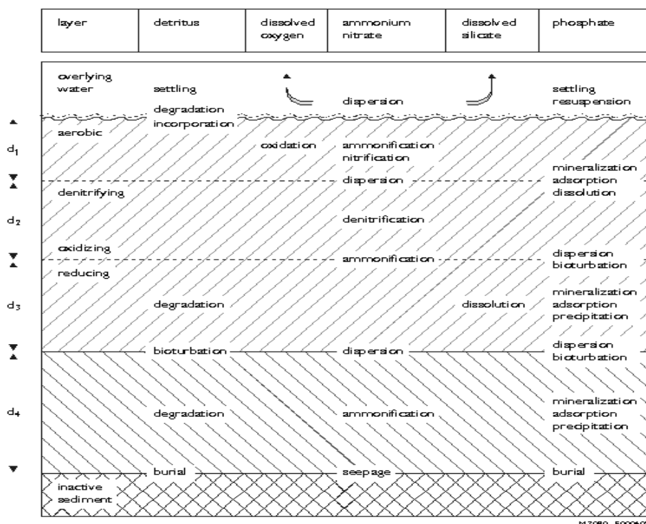
Figure 2.2: Overview of the processes included in SWITCH
